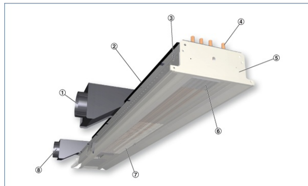
Schematic illustration of DID300B
